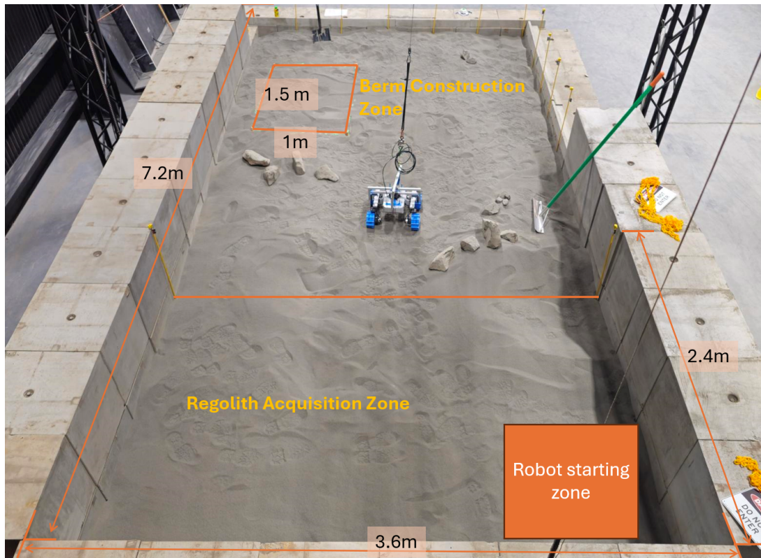
Figure 8.1.: Schematic of indicative indoor simulated lunar arena (note that dimensions, zone locations, and obstacles will all be significantly updated for ARCH 2027)
