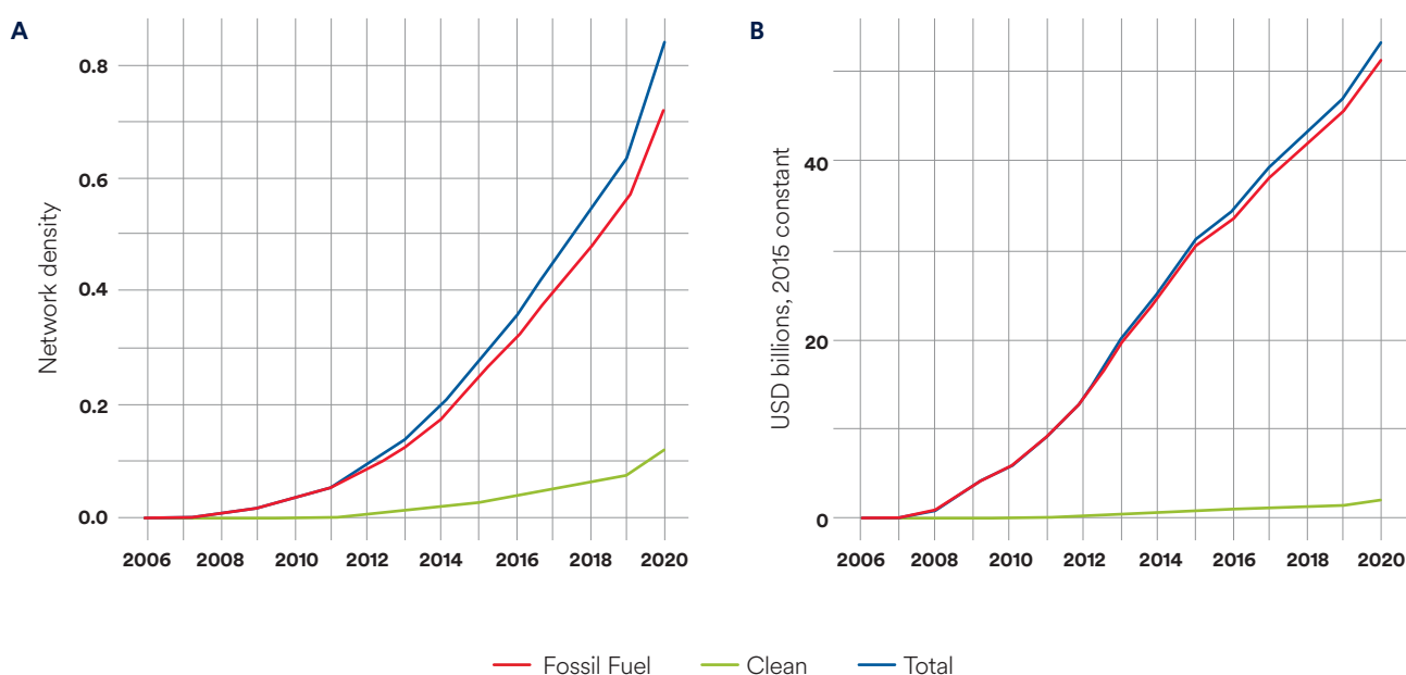
Figure 1: Network Density and average weighted degree
