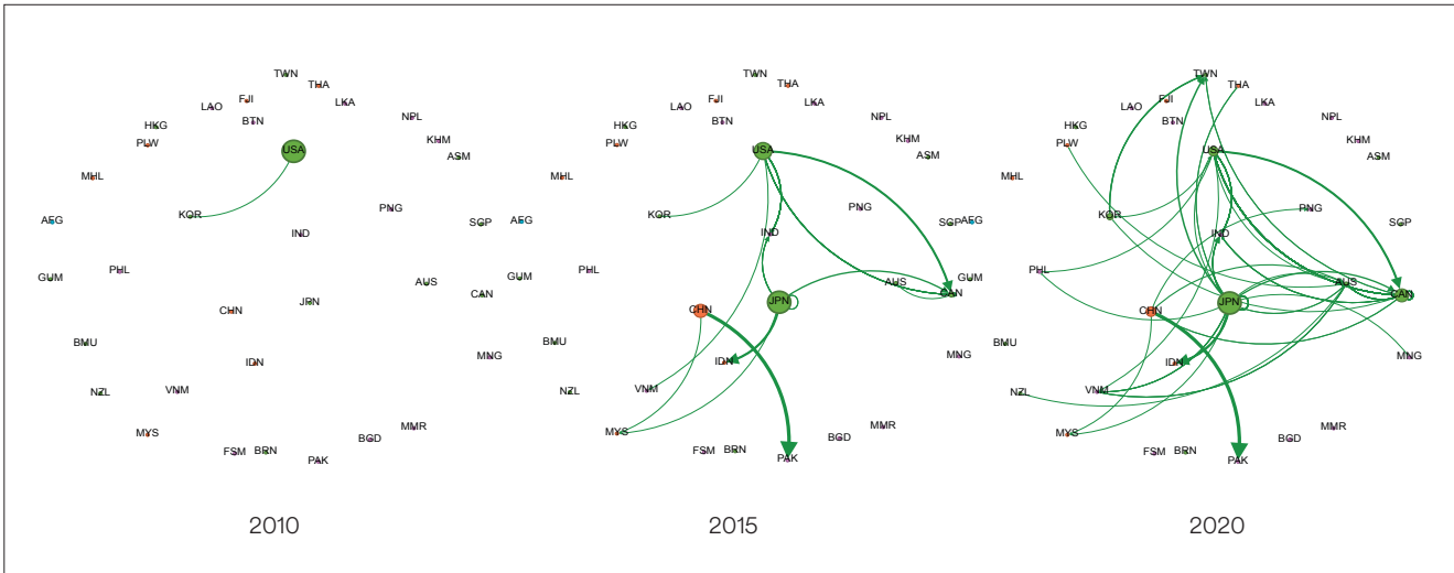
Figure 4: Evolution of the clean energy network
