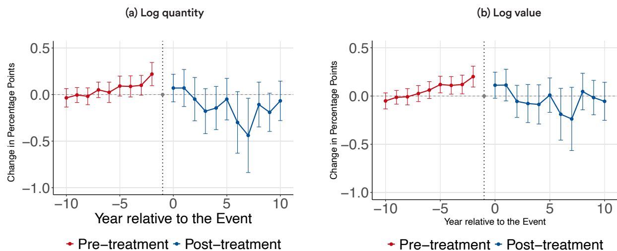
Figure 10: Event-study: baseline
